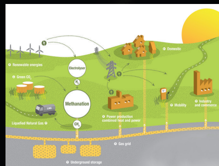
Power-to-gas couples various elements of the energy system
